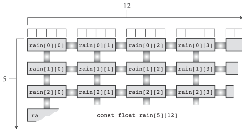
Figure 10.1 Two-dimensional array.
